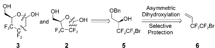
Scheme 1. Retrosynthetic analysis for 2 and 3 .
